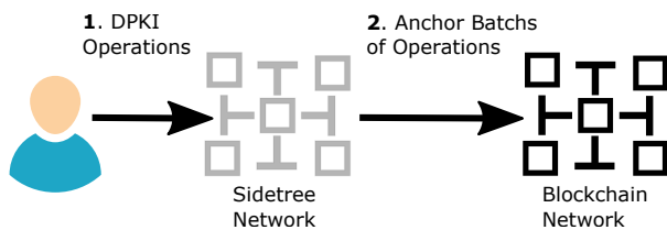
Fig. 4. DPKI using the Sidetree protocol
