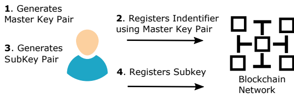
Fig. 3. DPKI Identifier and public keys registration
