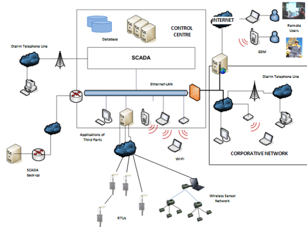
Fig. 1. A SCADA network architecture
