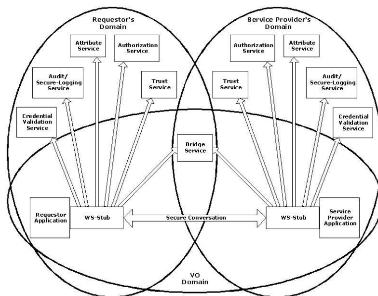
Figure 3: Security services in a virtual organization setting.
