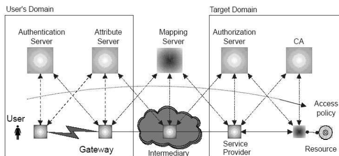
Figure 2: A service request scenario involving intermediaries.
