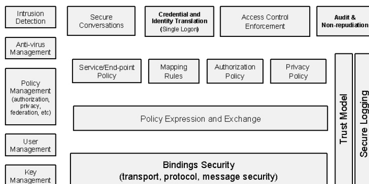
Figure 4: Components of Grid Security Model.
