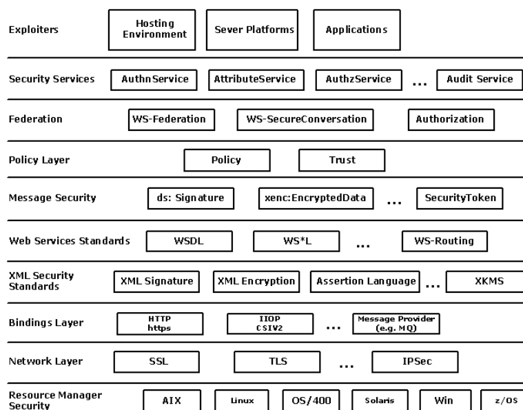
Figure 5: Security Specifications "Stack".
