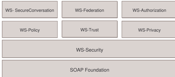
Figure 1: WS-Security model.
