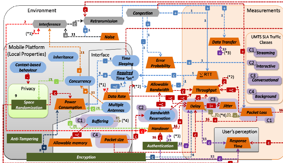
Fig. 2. Security and QoS Parametric Relationships in Mobile Platform
